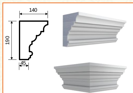
K-22 (190x140x2000)
