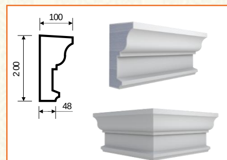
T-24 (200x100x2000)
