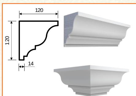
К-1 (120x120x2000)
