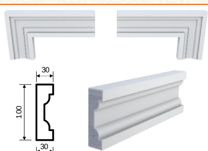
M-7 (100x30x2000)
