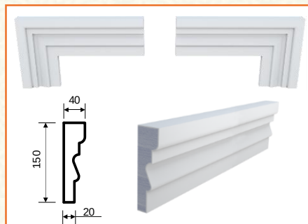
M-35 (150x40x2000)
