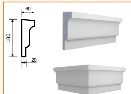
T-9 (180x60x2000)
