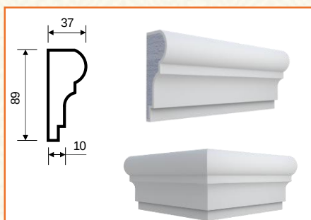
T-2 (89x37x2000)
