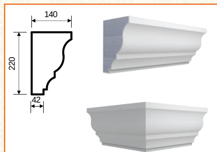
K-15 (220x140x2000)
