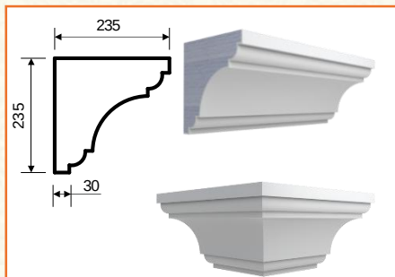
K-18 (235x235x2000)
