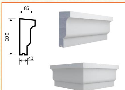
T-11 (200x85x2000)
