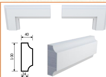
M-9 (100x40x2000)
