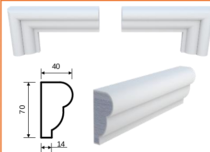
M-3 (70x40x2000)
