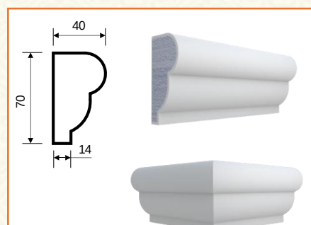
T-15 (70x40x2000)
