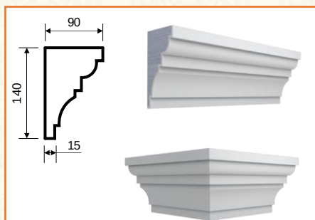
K-20 (140x90x2000)
