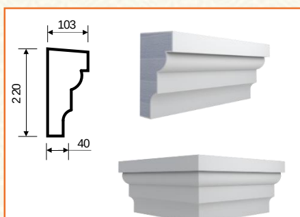
T-14 (220x103x2000)
