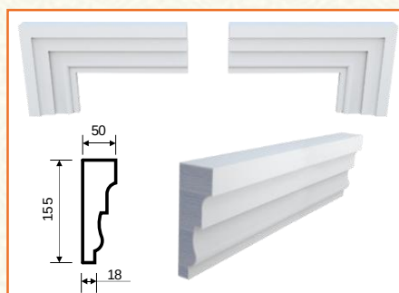
M-38 (155x50x2000)
