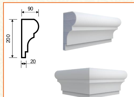
T-12 (200x90x2000)
