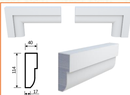
M-12 (114x40x2000)
