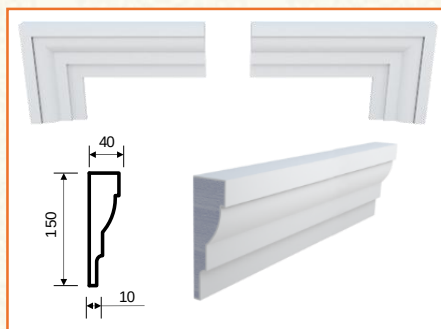
M-31 (150x40x2000)
