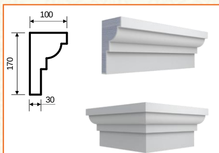
K-21 (170x100x2000)
