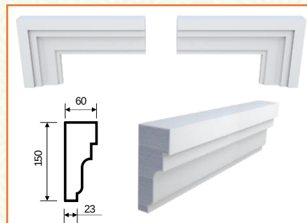
M-36 (150x60x2000)
