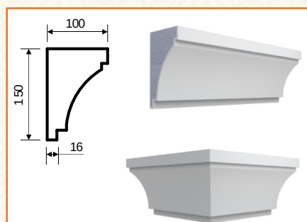
К-3 (150x100x2000)
