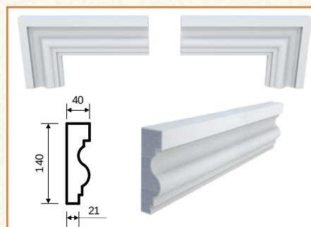
M-45 (140x40x2000)
