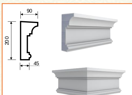
T-13 (200x90x2000)
