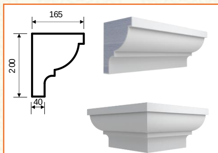
K-12 (200x165x2000)
