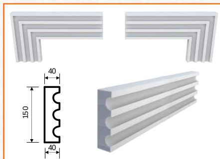
M-34 (150x40x2000)
